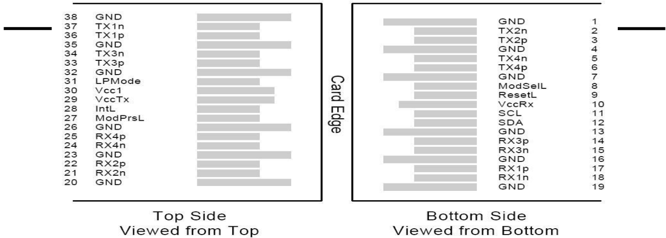
Figure3. Electrical Pin-out Details
