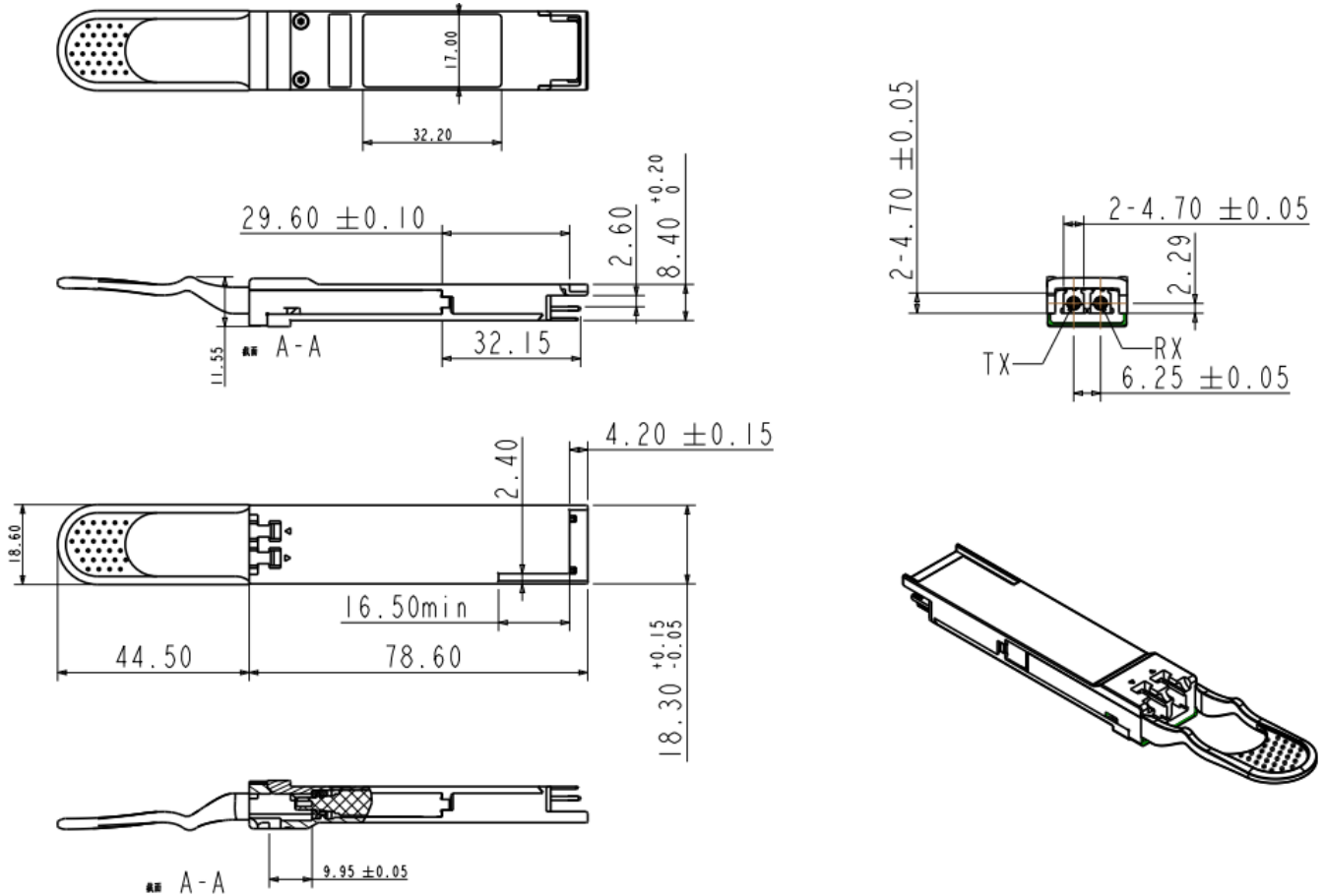
Figure 9 . Mechanical Specifications
